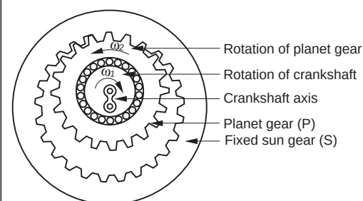
Fig.F-2 Epitrochoid Planet Gear-Circular (PIN) Tooth Sun Gear Combination
