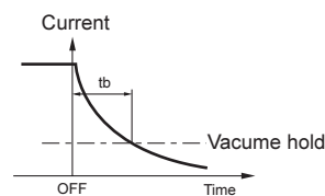
Fig. F-35 Current Curve of Standard Braking
