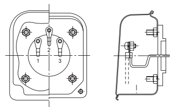
3-Phase indoor terminal box
