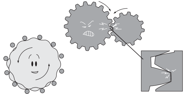
CYCLO® DRIVE has smooth rolling contact.
