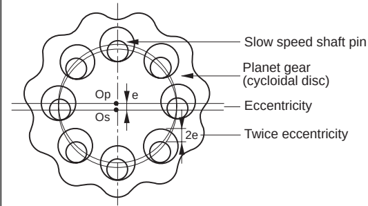
Fig.F-4 Combination of Planet-Sun Gears and Constant Speed Internal Gear
