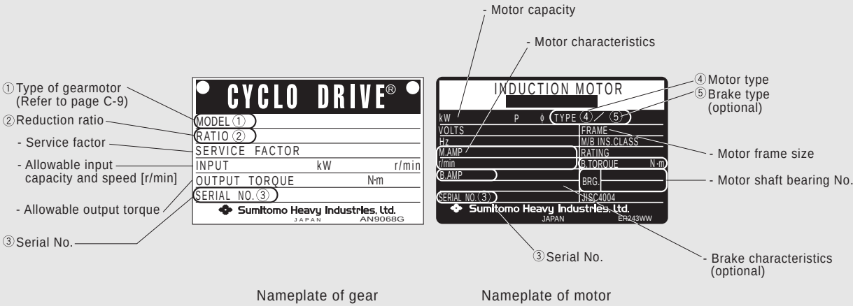
Fig. F-6 Nameplates of Reducer with Motor (Type II)
